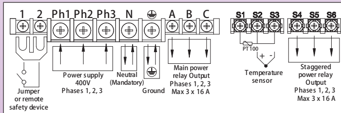
3 pole circuits, 2 staggered relay outputs 3x16A 250V
